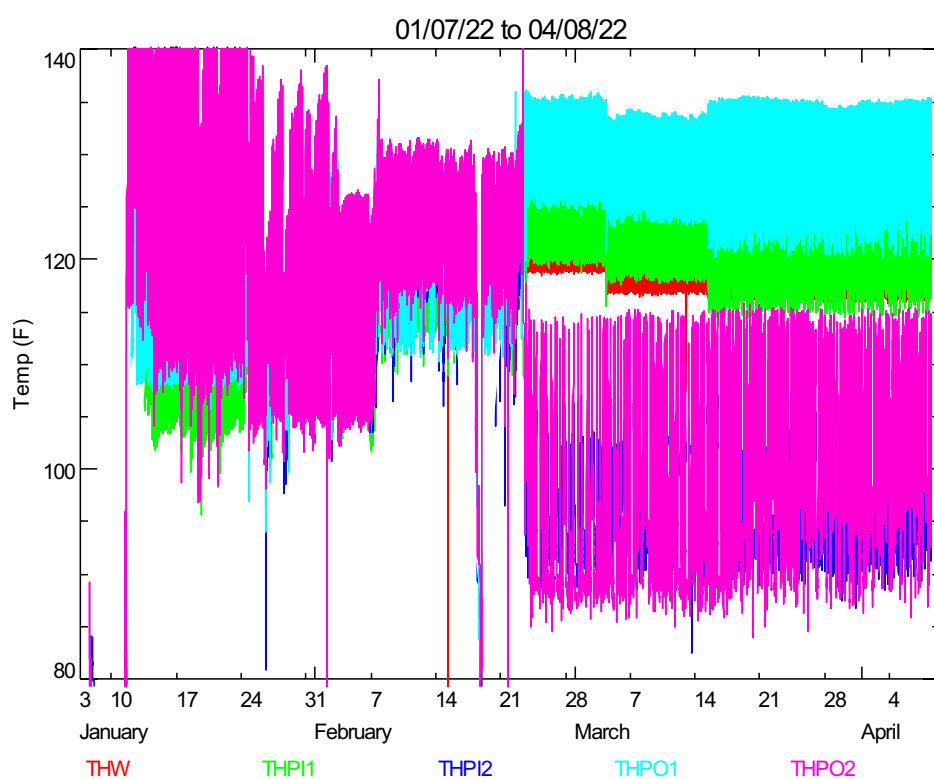
Figure 21. Initial Operating Temperatures for the DHW System in Early 2022
