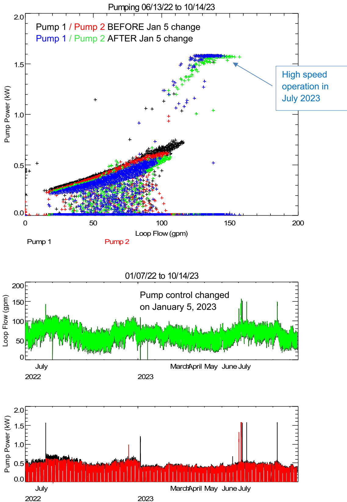
Figure 15. Trends of Pumping Power and Ground Loop Flow
