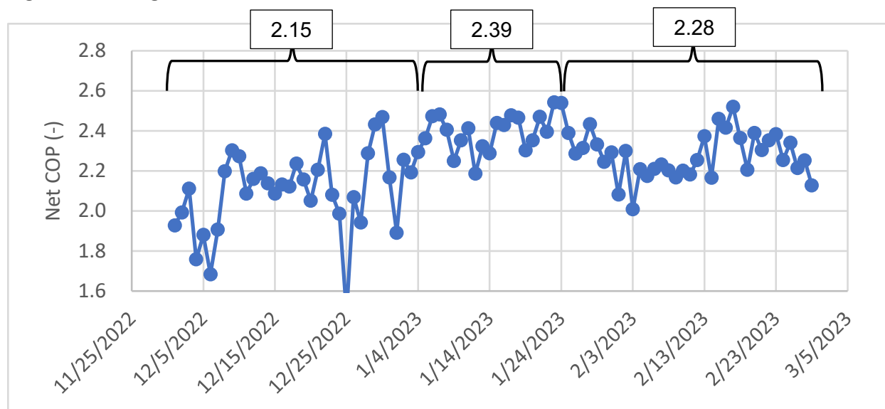
Figure 31. Change in Net COP Between Periods Listed in Table 10
