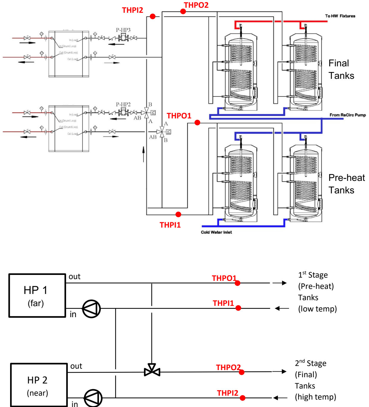
Figure 9. Schematic of WWHP and Storage Tanks with Monitoring Points Shown
