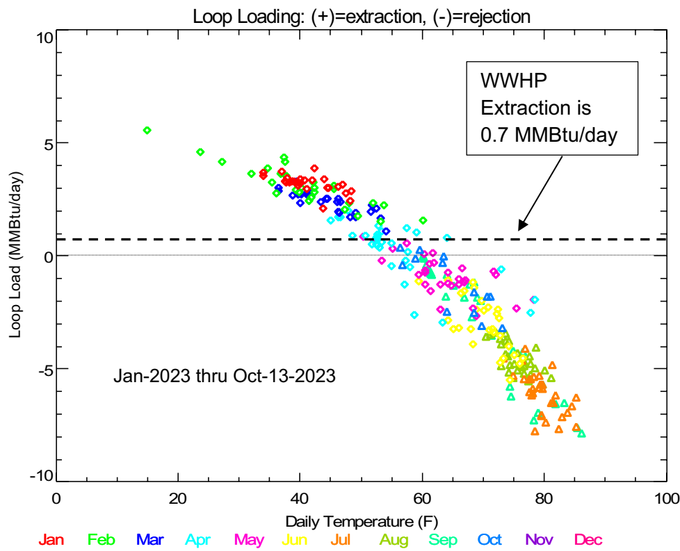
Figure 18. Daily Ground Loop Loading versus Daily Outdoor Temperature
