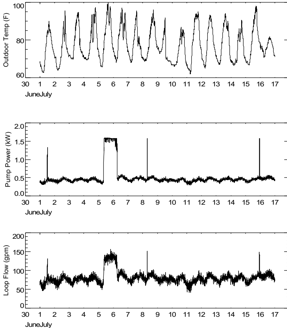
Figure 16. Trend of Pumping Power and Ground Loop Flow in July 2023
