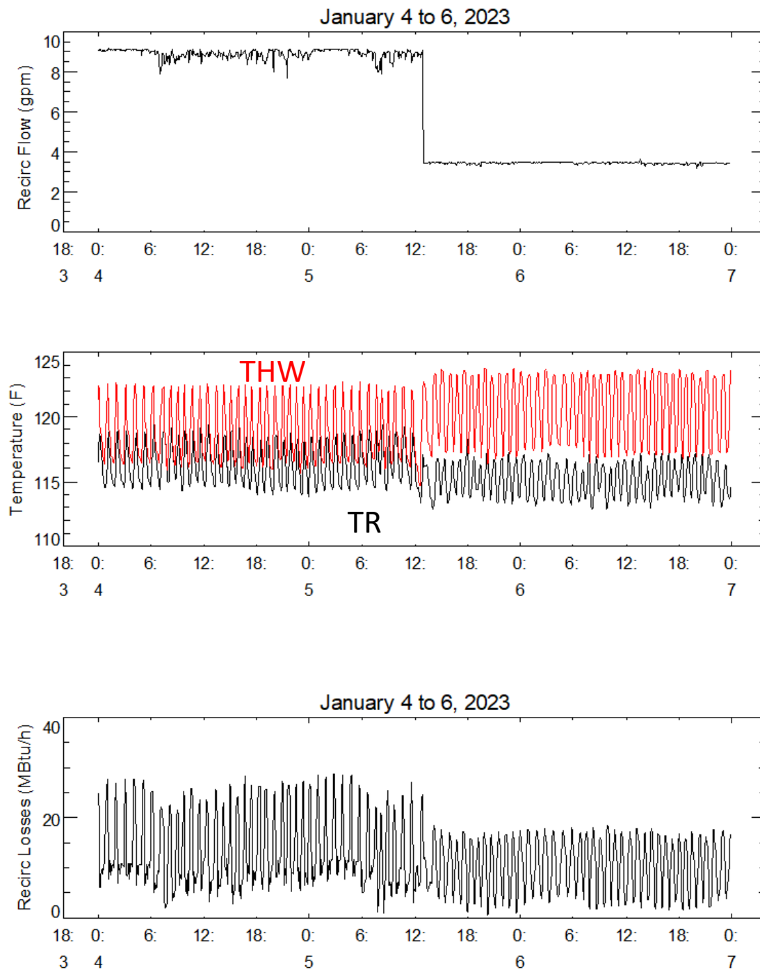
Figure 29. Impact of Reduced Recirculation Flow on January 5, 2023
