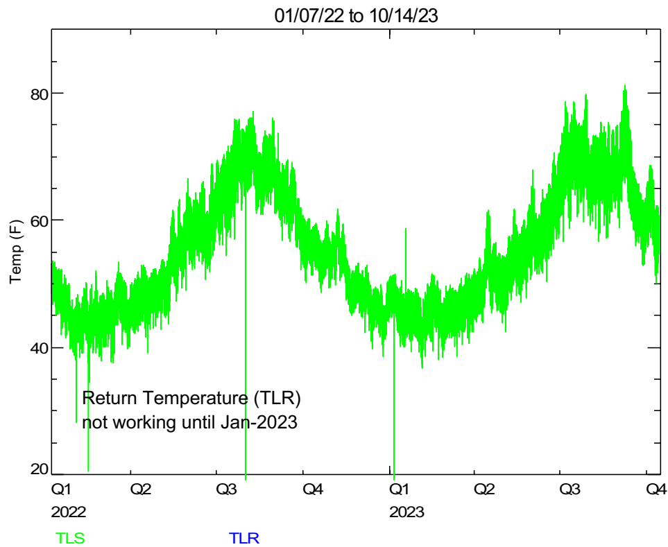
Figure 12. Trend of Ground Loop Supply Temperatures (TLS), Loop Flows, and Loop Delta-T Over the Monitoring Period
