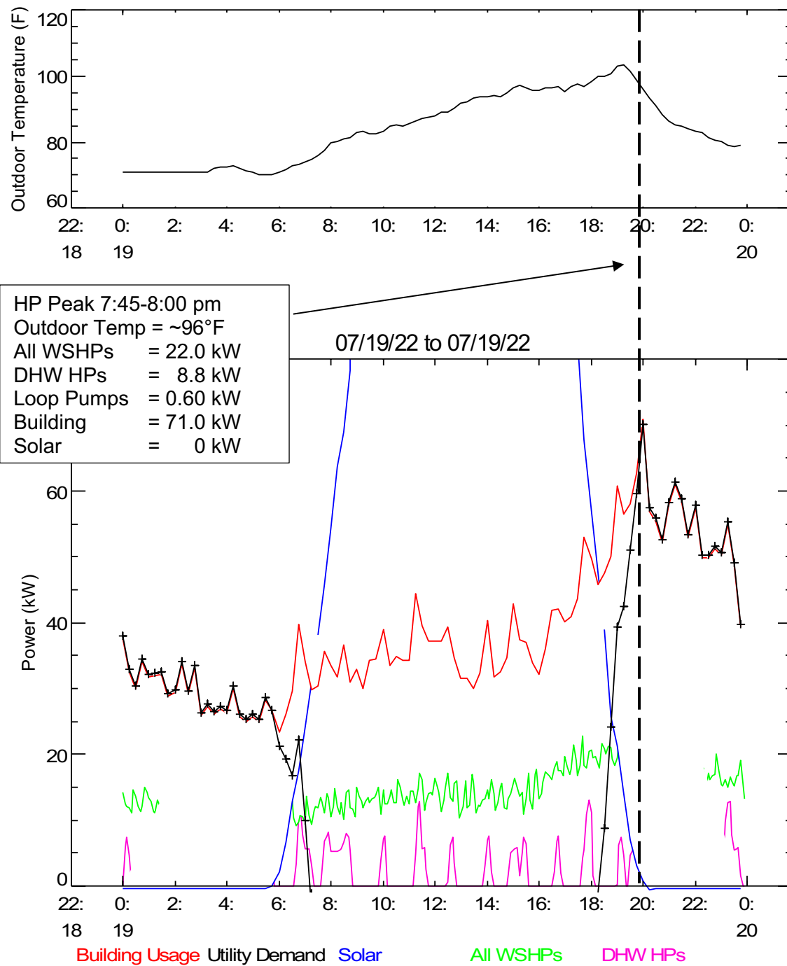
Figure 33. Building and HVAC Demand on the Hottest Day – July 19, 2023
