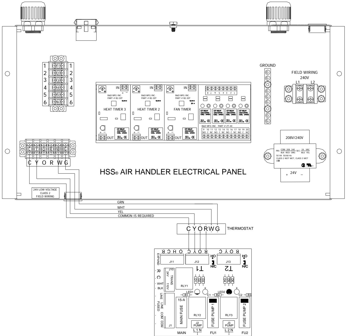
HSS® BUFFER TANK B3-6CR BOARD
