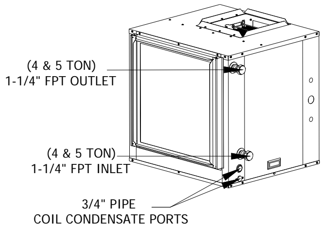
4 TON & 5 TON HSS® AIR HANDLER PIPING CONNECTIONS
